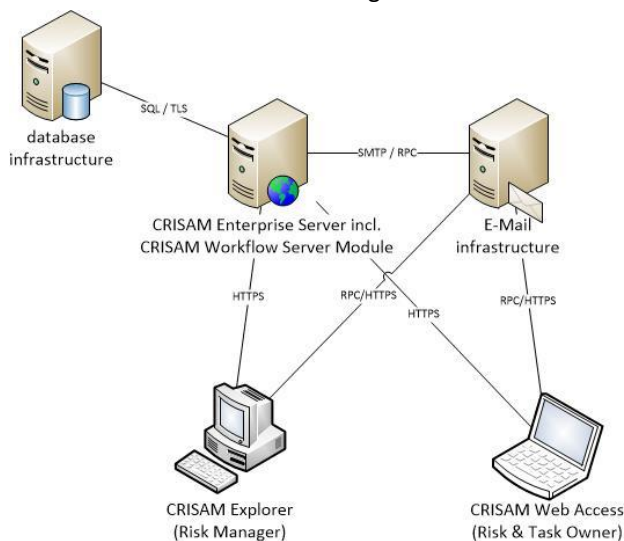
Figure 1 - system architecture
